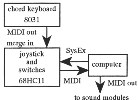
Figure 5: Controller electronics
